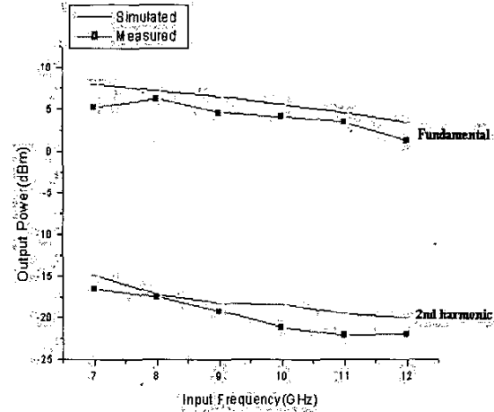
Fig. 5 Measured and simulated doubler output power versus frequency. Input power is -5dBm
