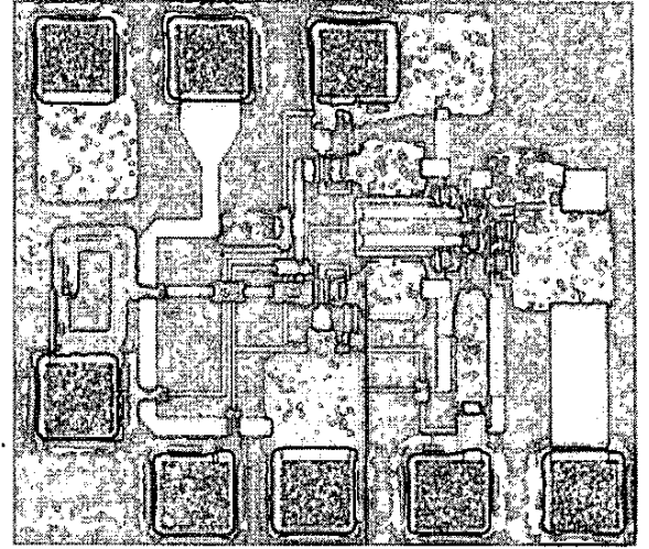
Fig. 3. Microphotograph of the balanced frequency doubler .
